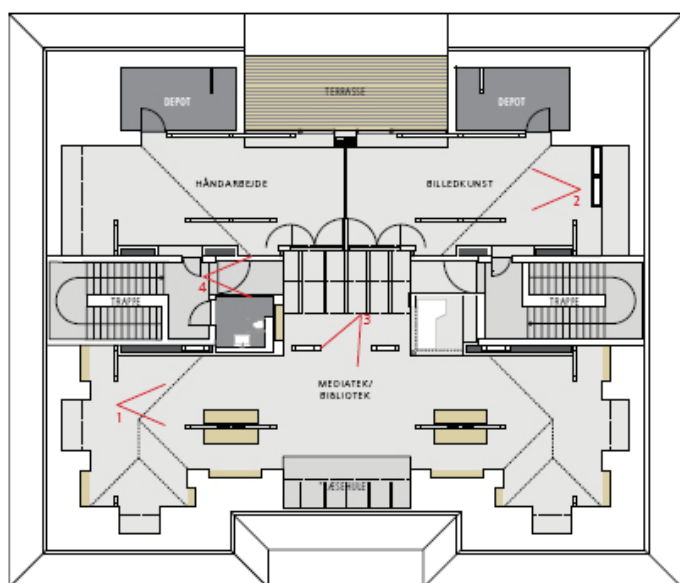
Plan 1:200
